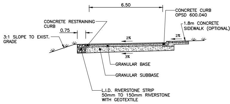
SECTION A-A (TYPICAL ROAD SECTION) N.T.S.
